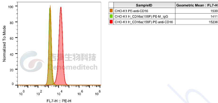
Figure 1 | H_FCGR3A(CD16a) 158F CHO-K1 Cell Line was determined by flow cytometry using PE anti-human CD16 Antibody (biologend/302007).
